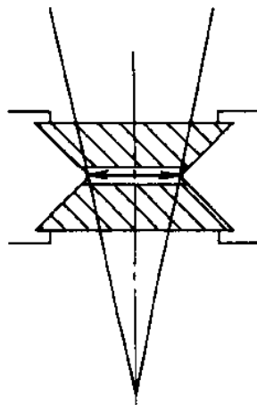
c. Double Conical (Withstands Two-Way Pressure)
