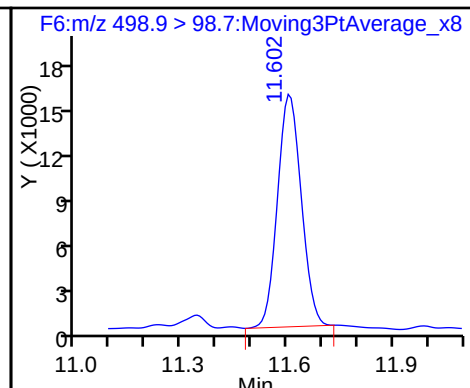
21 PFNS (Perfluoro-1-nonanesulfonate)
