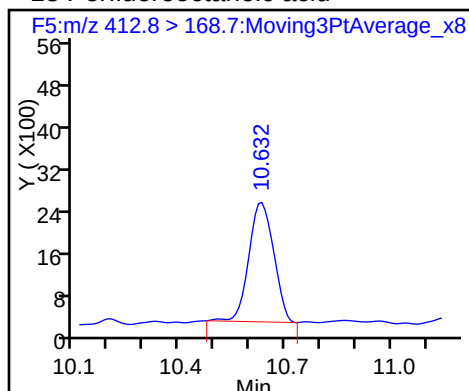
15 Perfluorooctanoic Sulfonate
