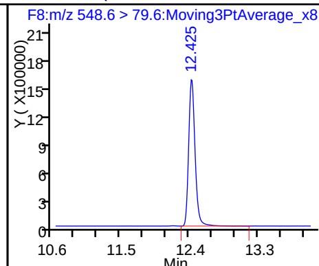
21 PFNS (Perfluoro-1-nonanesulfonate)
