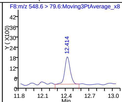
21 PFNS (Perfluoro-1-nonanesulfonate)
