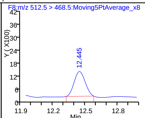
21 PFNS (Perfluoro-1-nonanesulfonate)
