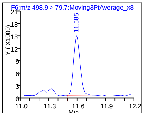
18 Perfluorononanoic acid
