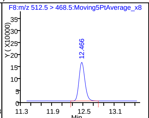
21 PFNS (Perfluoro-1-nonanesulfonate)
