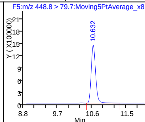
15 Perfluorooctanoic Sulfonate
