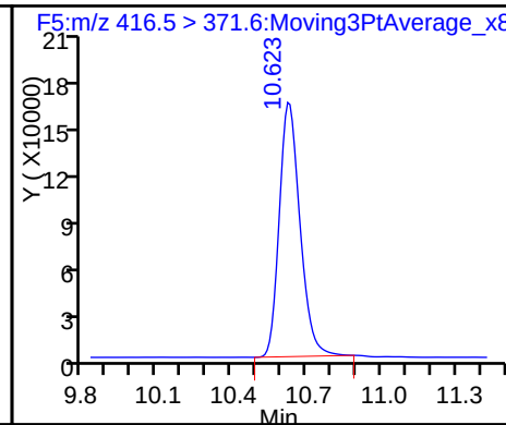
14 Perfluoroheptane Sulfonate
