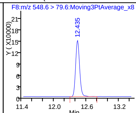
21 PFNS (Perfluoro-1-nonanesulfonate)
