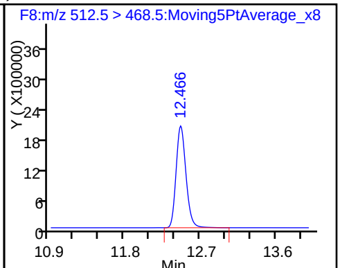
21 PFNS (Perfluoro-1-nonanesulfonate)
