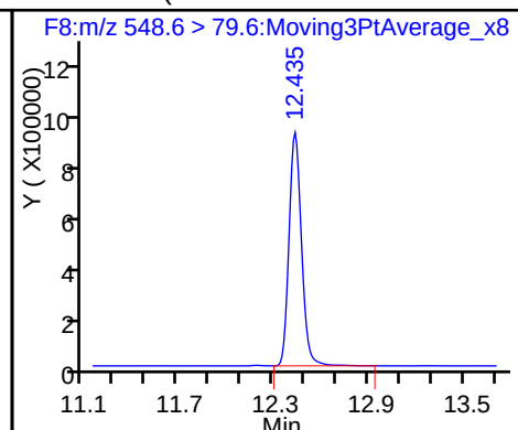
21 PFNS (Perfluoro-1-nonanesulfonate)
