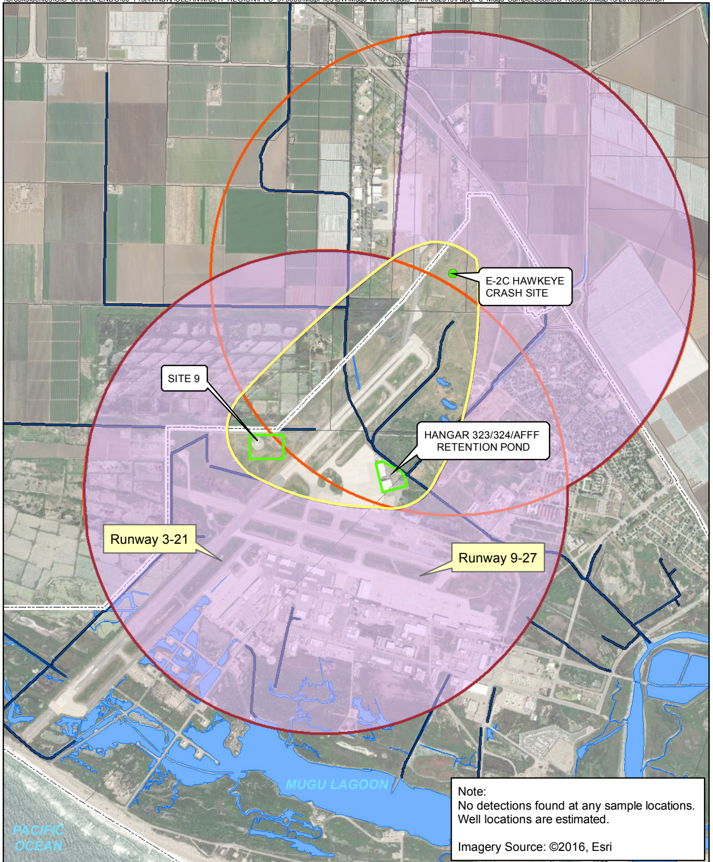
Figure 3 Sample Location Map and Results Site 9, Hangar 323/324/AFFF Retention Pond, and E-2C Hawkeye Crash Naval Base Ventura County Point Mugu Ventura County, California
