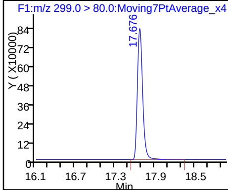
4 Perfluoroheptanoic acid
