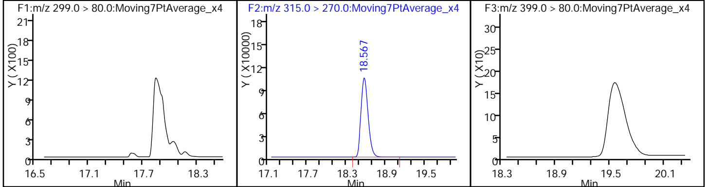
4 Perfluoroheptanoic acid
