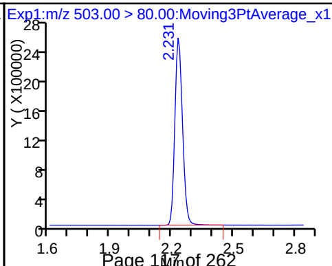
8 Perfluorooctane sulfonic acid (ND) * 7 13C4 PFOS
