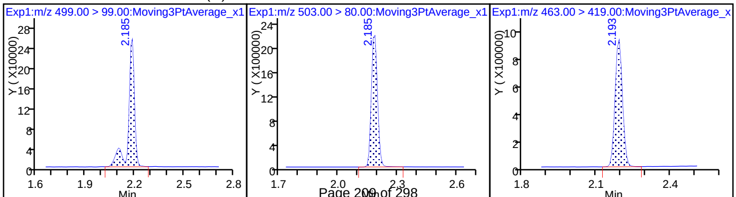
9 Perfluorononanoic acid
